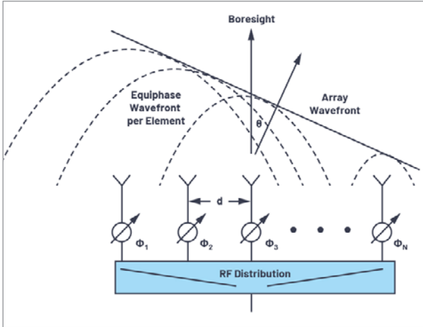
2. This phased-array arrangement uses phase shifters rather than time delay.
