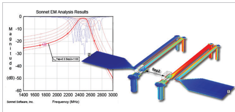
3. Sonnet Lite is a free version of the 3D EM simulator for analysis of planar structures such as coupled transmission lines. (Courtesy of Sonnet Software)
