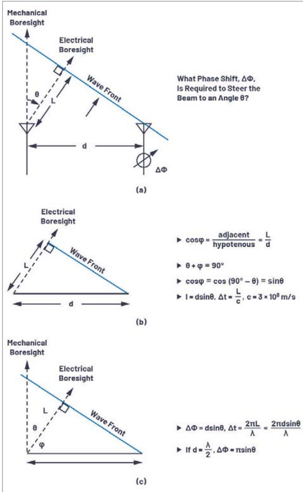
3. To visualize the phase shift needed for beamsteering, a set of right triangles can be drawn between adjacent elements, where \Delta\Phi is the phase shift between those adjacent elements.
