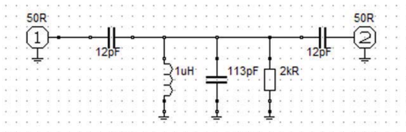
3. Shown is the 2-port example circuit used for VNA measurements.
