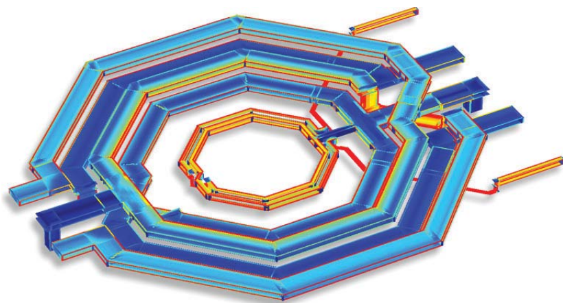
1. Many EM simulators provide the precision needed to study the fields around sections of passive circuit elements or semiconductor ICs. (Courtesy of Sonnet Software)
