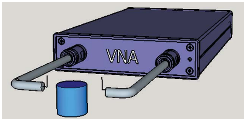
1. For a 2-port Q measurement of a resonator, establish very light input and output coupling to reduce the loading effect of the 50-Ω source and load impedances.
