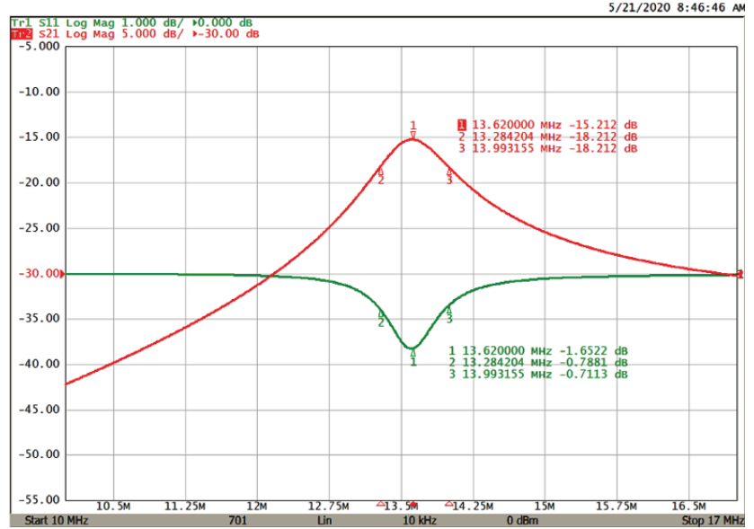
4. This graph illustrates a 3-dB Q factor measurement of the circuit shown in Figure 3.
