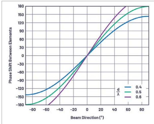
4. Shown are plots of phase shift ( \Delta\Phi ) between elements vs. beam direction ( \theta ) for three cases of d/\lambda .
