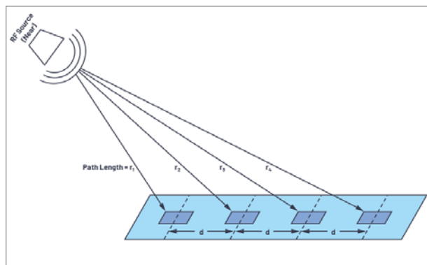
6. In the case of an RF source near the linear array, the angle of incidence varies for each element.
