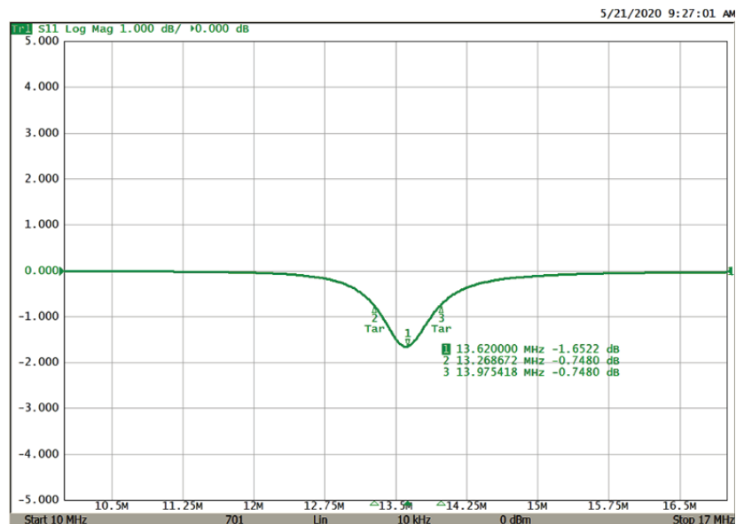
5. In this graph, we see the S_{11} measurement alone.
