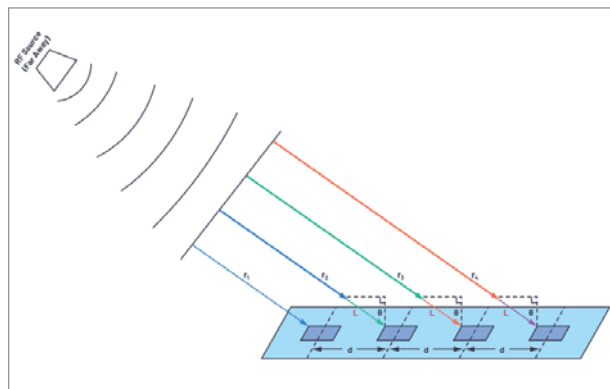
7. If the RF source is far away from the linear array, the large radius of the spherical wavefront results in wave propagation paths that are approximately parallel.
